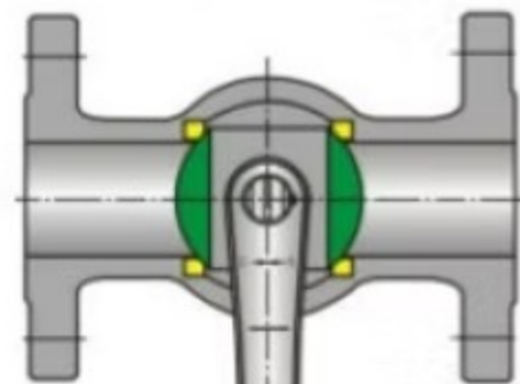
'OFF' Position
